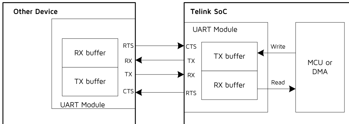
Figure 10-20 UART Communication
