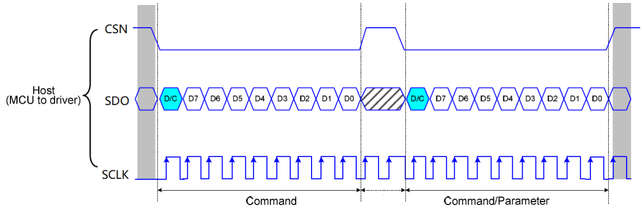
Figure 10-10 3-Line Read Sequence
