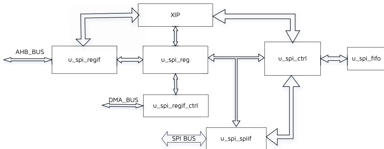
Figure 10-6 HSPI Diagram
