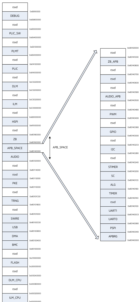
Figure 4-1 Memory Map
