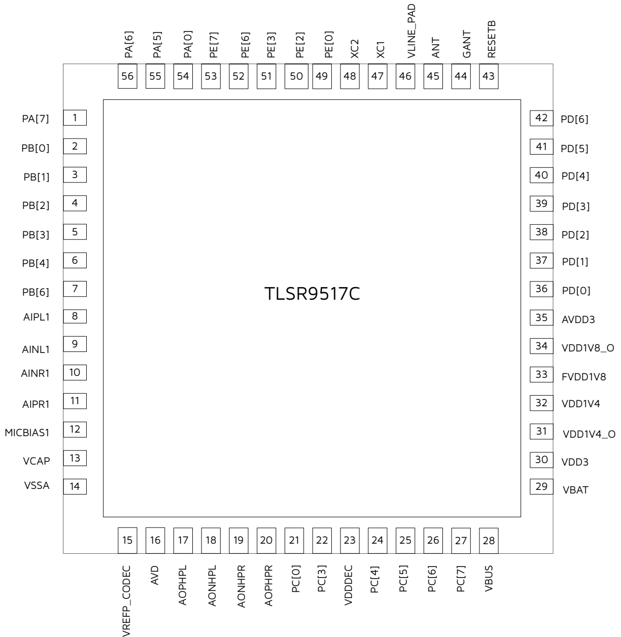
Figure 1-5 Pin Assignment of TLSR9517C
