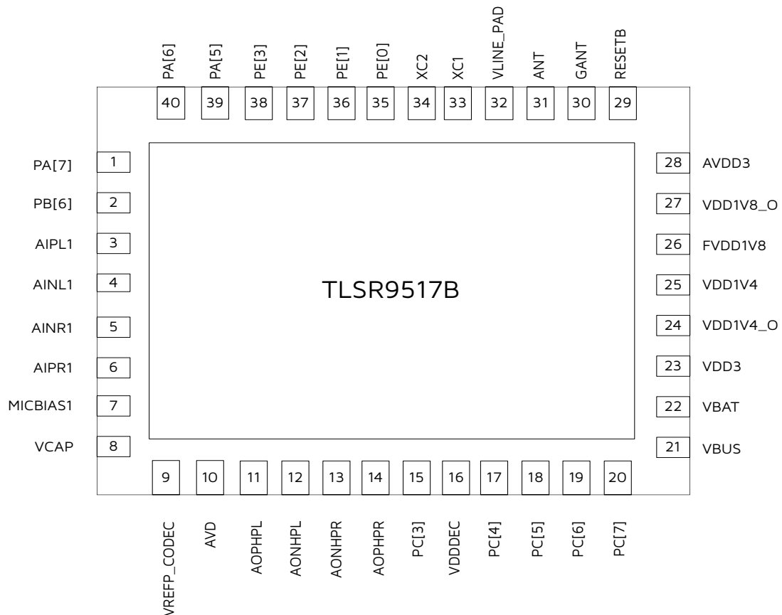
Figure 1-4 Pin Assignment of TLSR9517B
