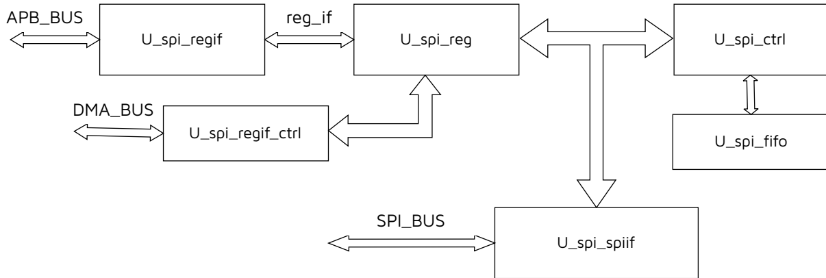
Figure 10-17 PSPI Diagram
