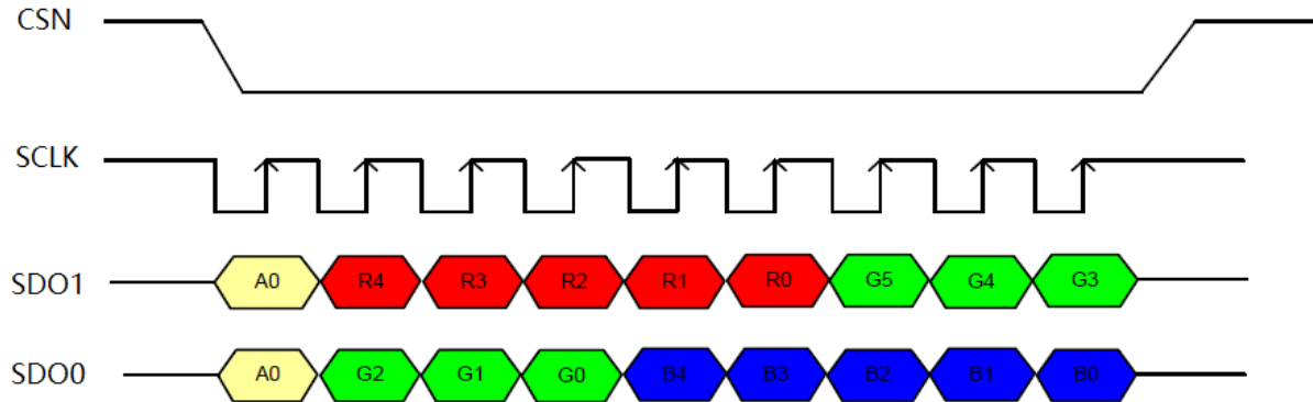
Figure 10-15 RGB666 Pixel Transition
